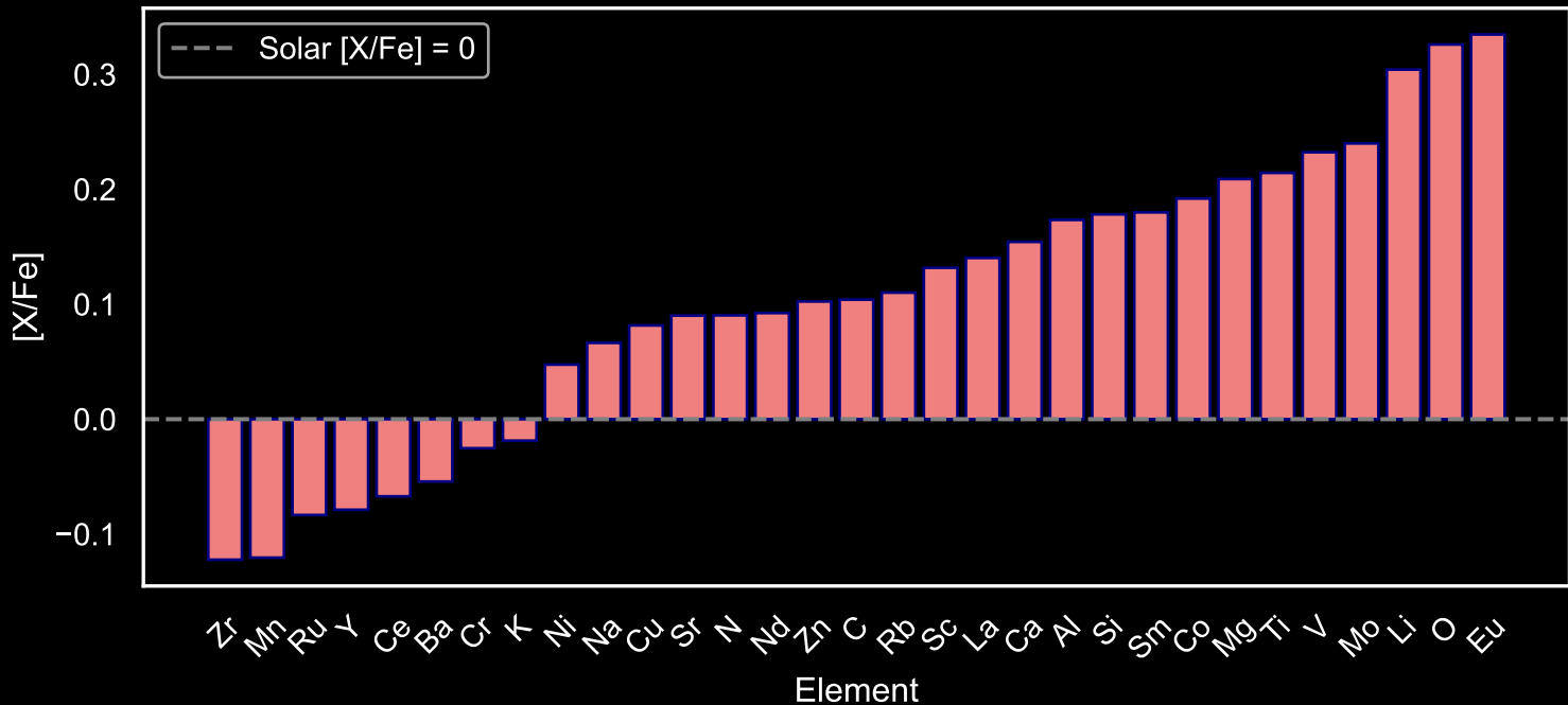
Abundance Pattern for GALAH Red Giants: Star Field [55] (N=78)
