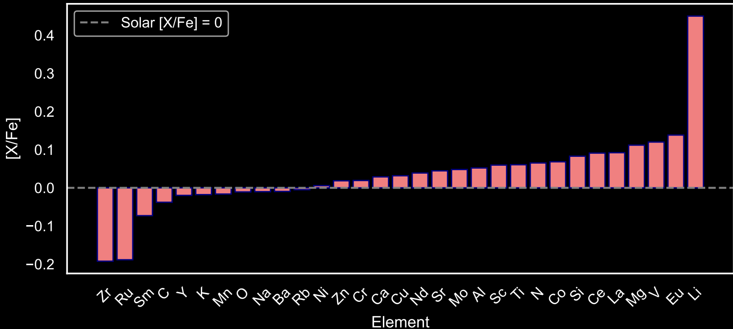
Abundance Pattern for GALAH Main Sequence Stars: Star Field [55] (N=148)
