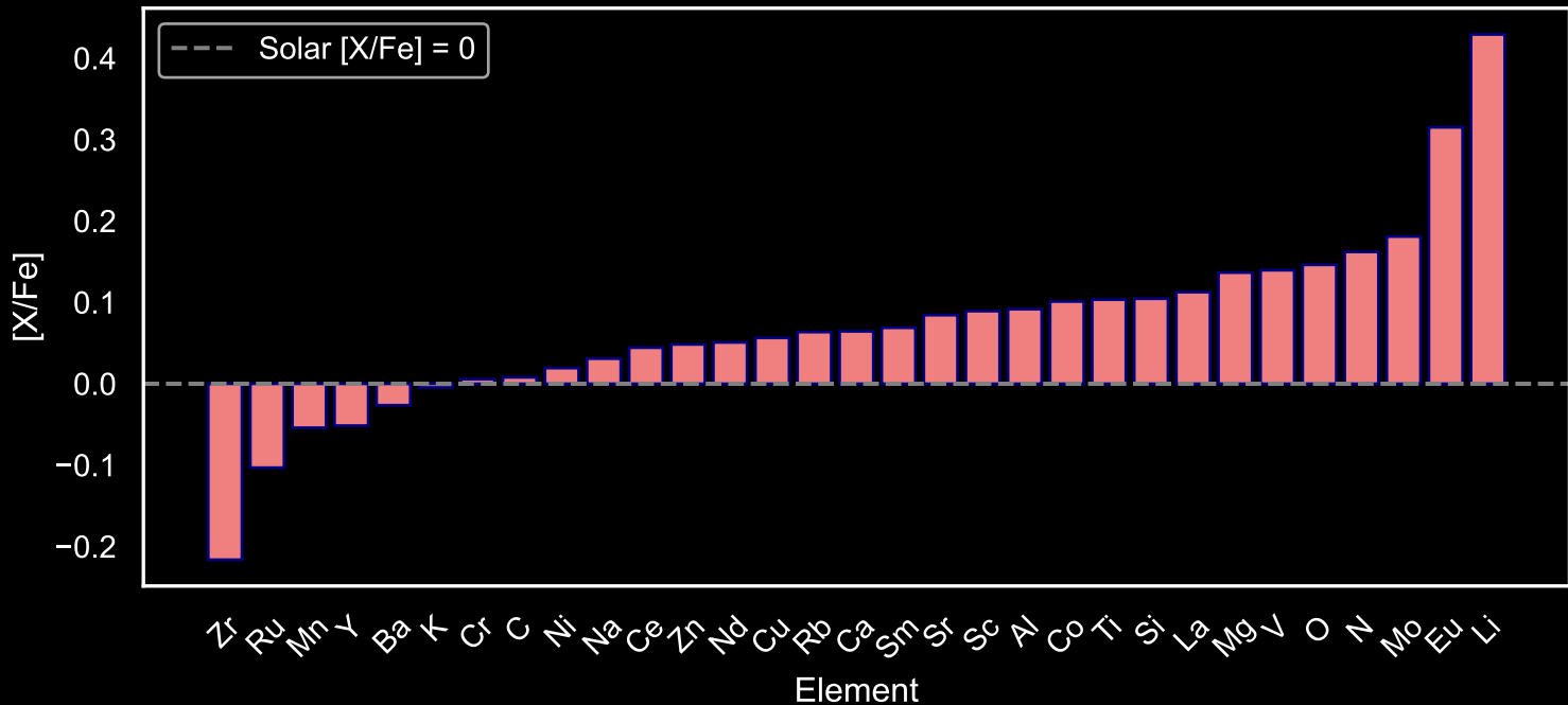
Abundance Pattern for GALAH Star Field [55] (N=322)
