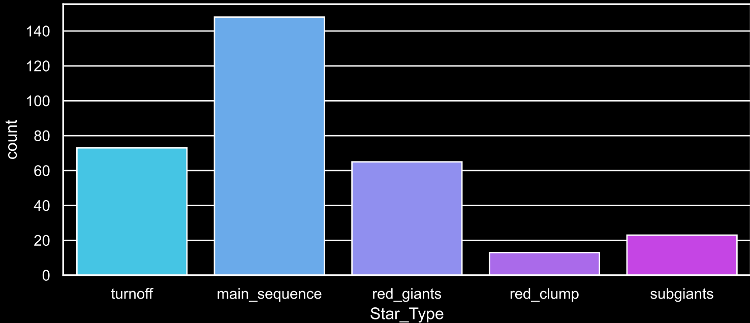
Field [55] Count plot of Star Type
